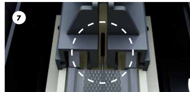
7 Make sure the contact wire from the lamp is straight between the contact plates inside the fitting
